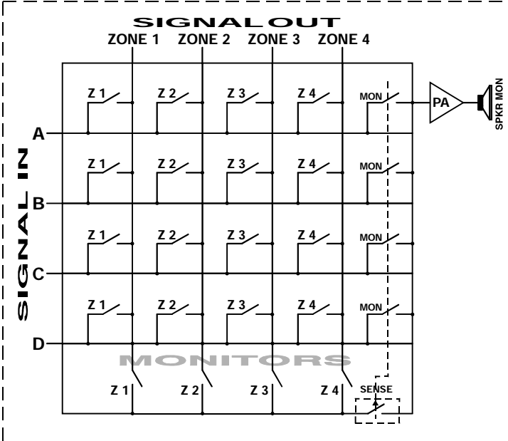
MMS 4004 FUNCTION DIAGRAM
